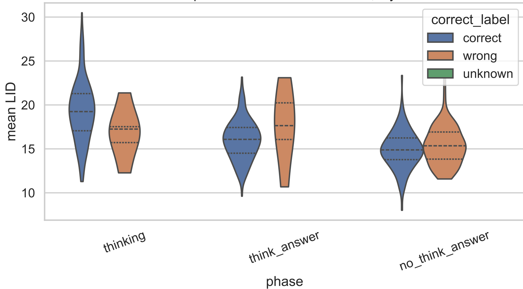
32B Exp C correctness-stratified LID, layer 6
