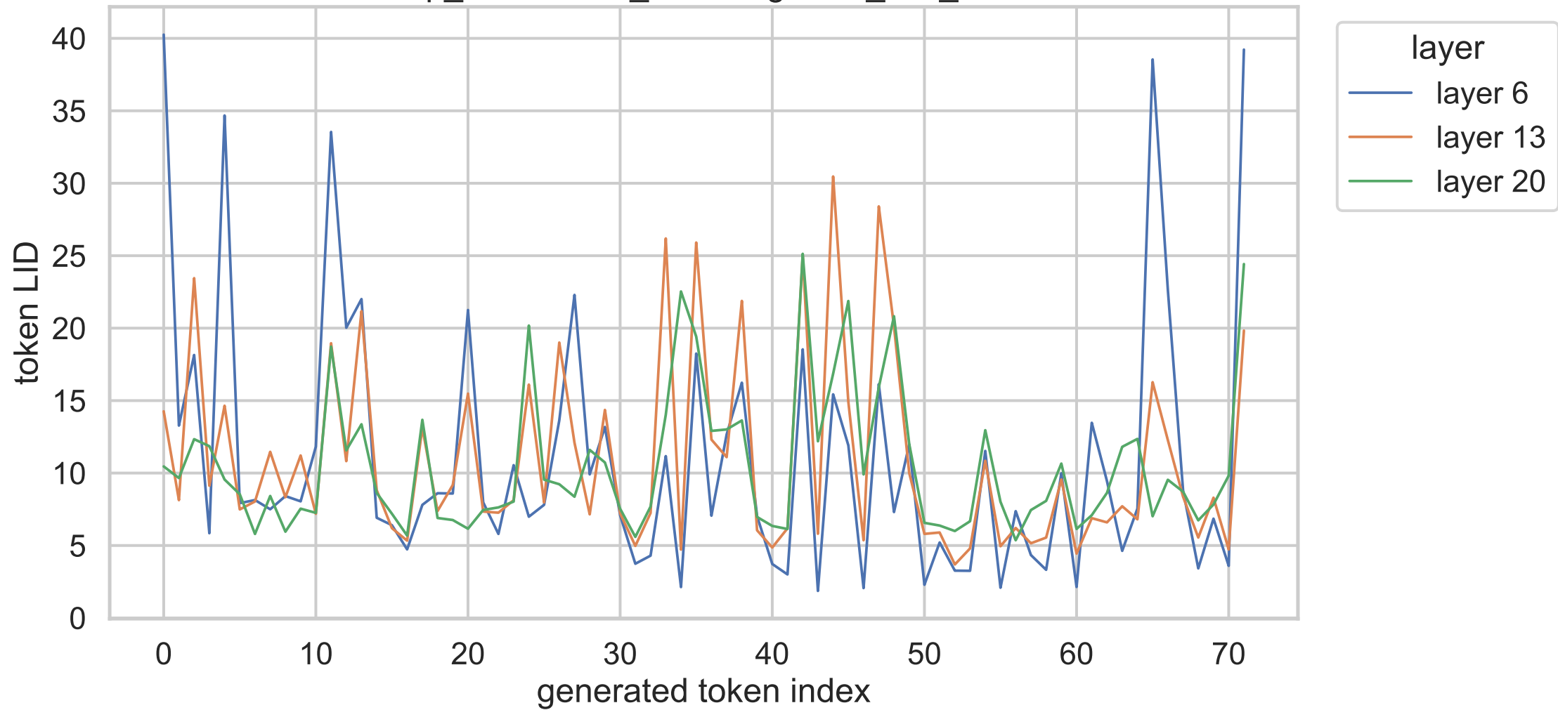
4B exp_b irrelevant_context_gsm8k_test_001130
