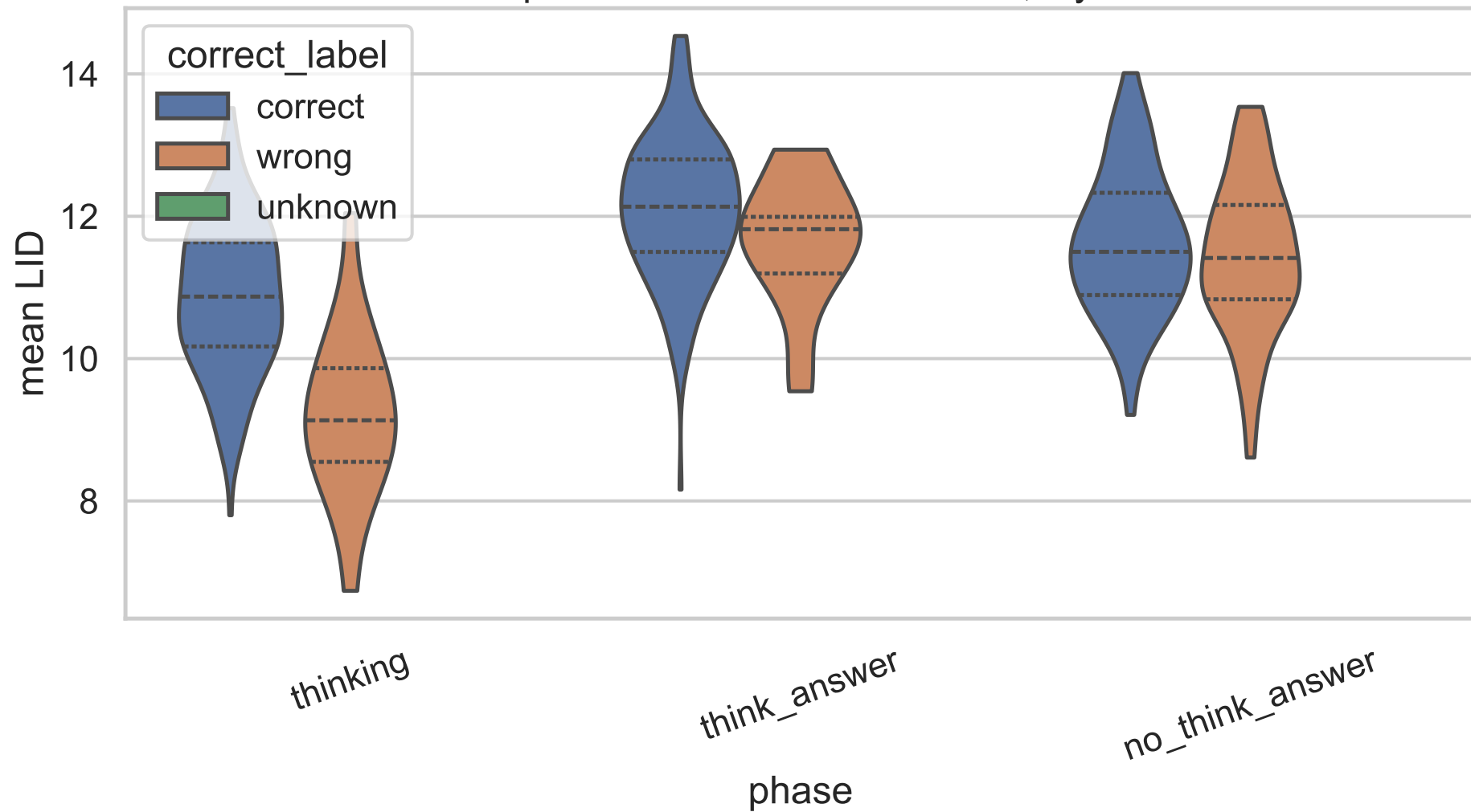
4B Exp C correctness-stratified LID, layer 13
