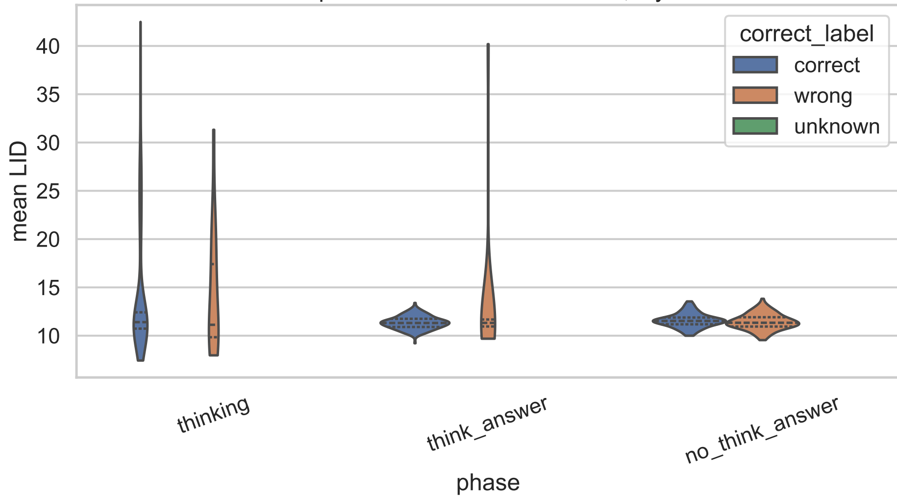
4B Exp C correctness-stratified LID, layer 20
