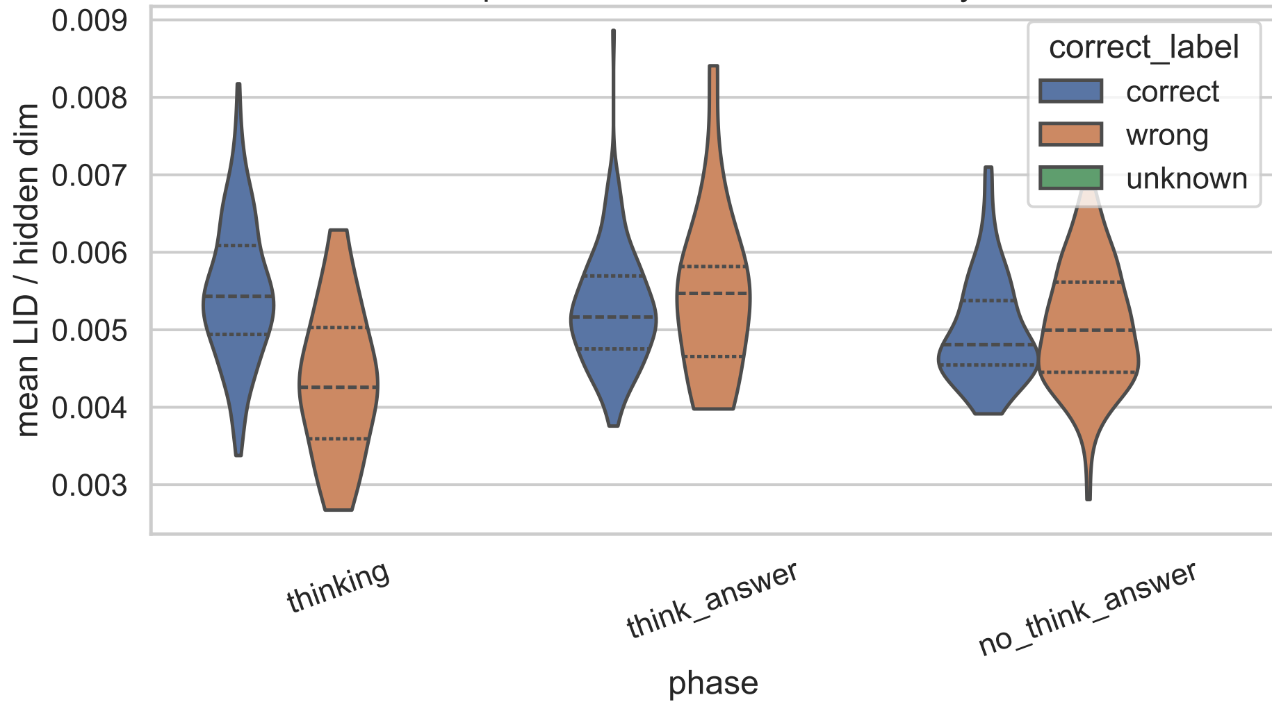
4B Exp C correctness-stratified LID, layer 6
