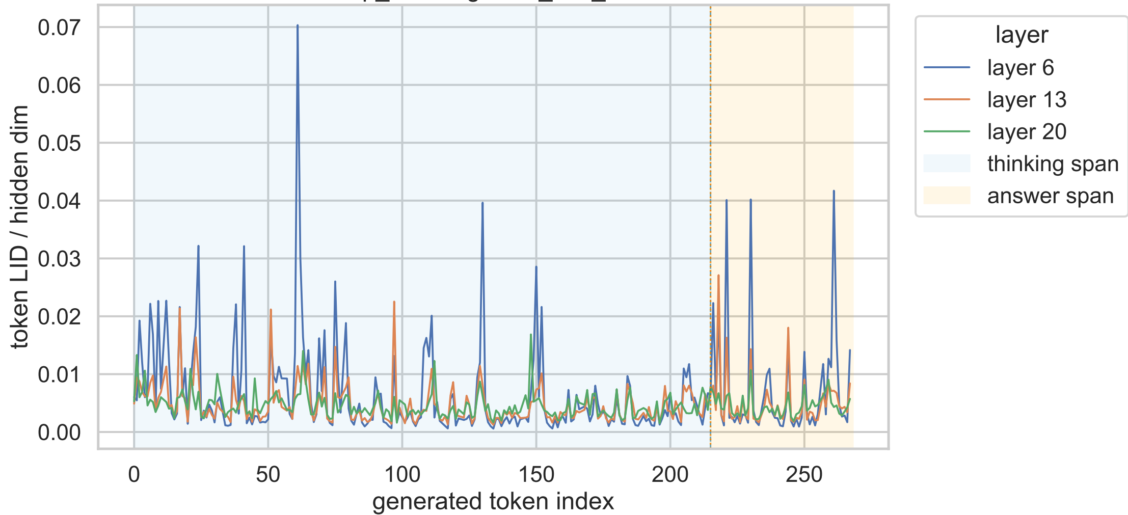
4B exp_c think gsm8k_test_001271
