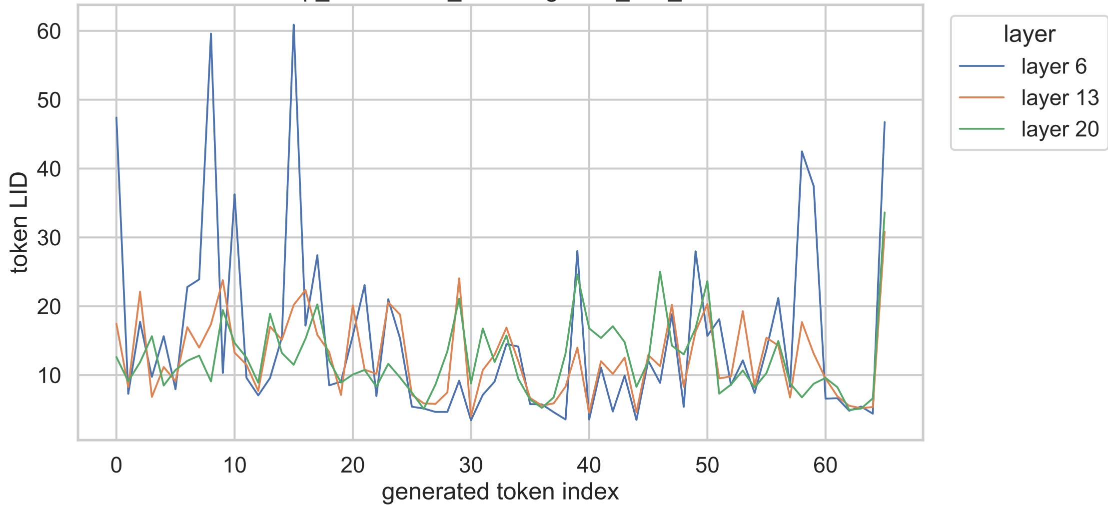
8B exp_b irrelevant_context gsm8k_test_001130
