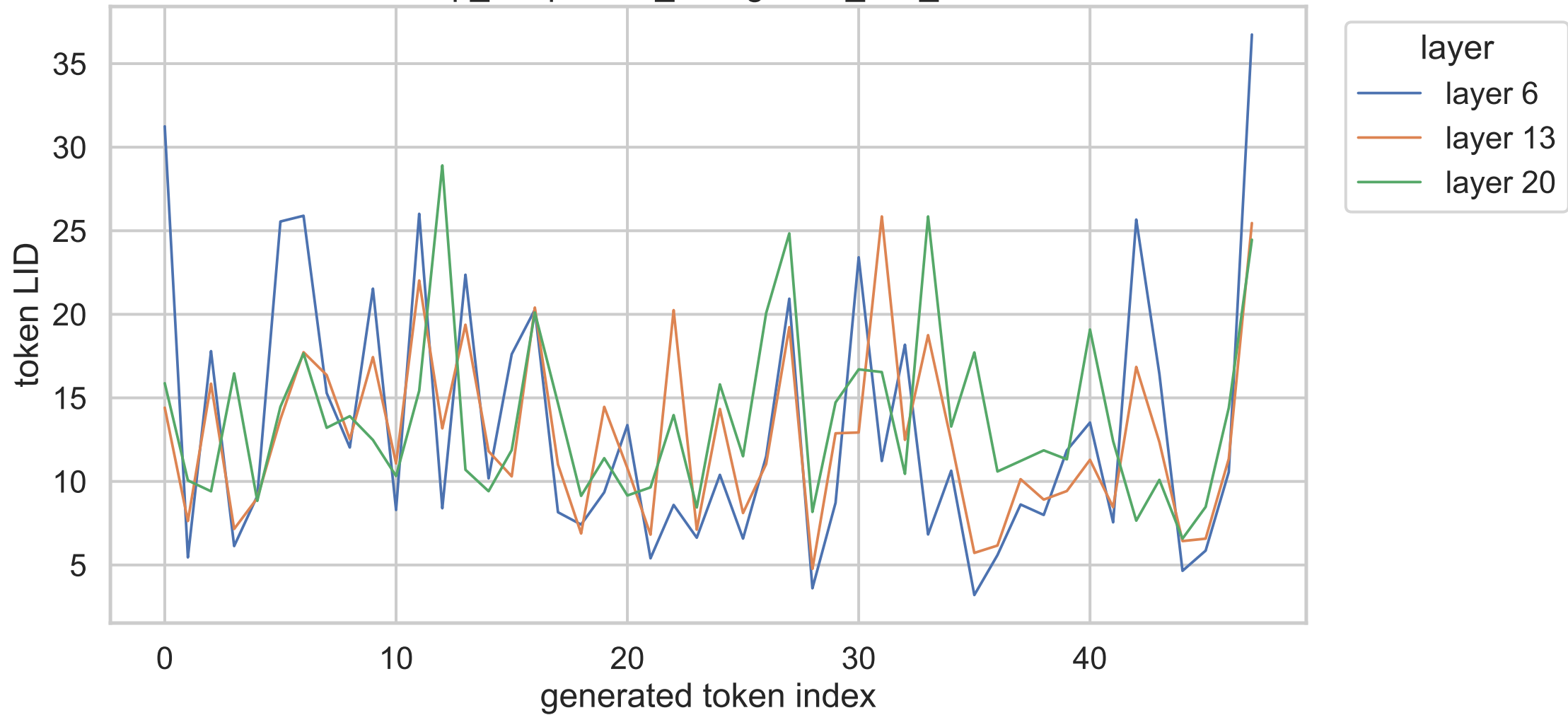
8B exp_b repetitive_filler gsm8k_test_000486
