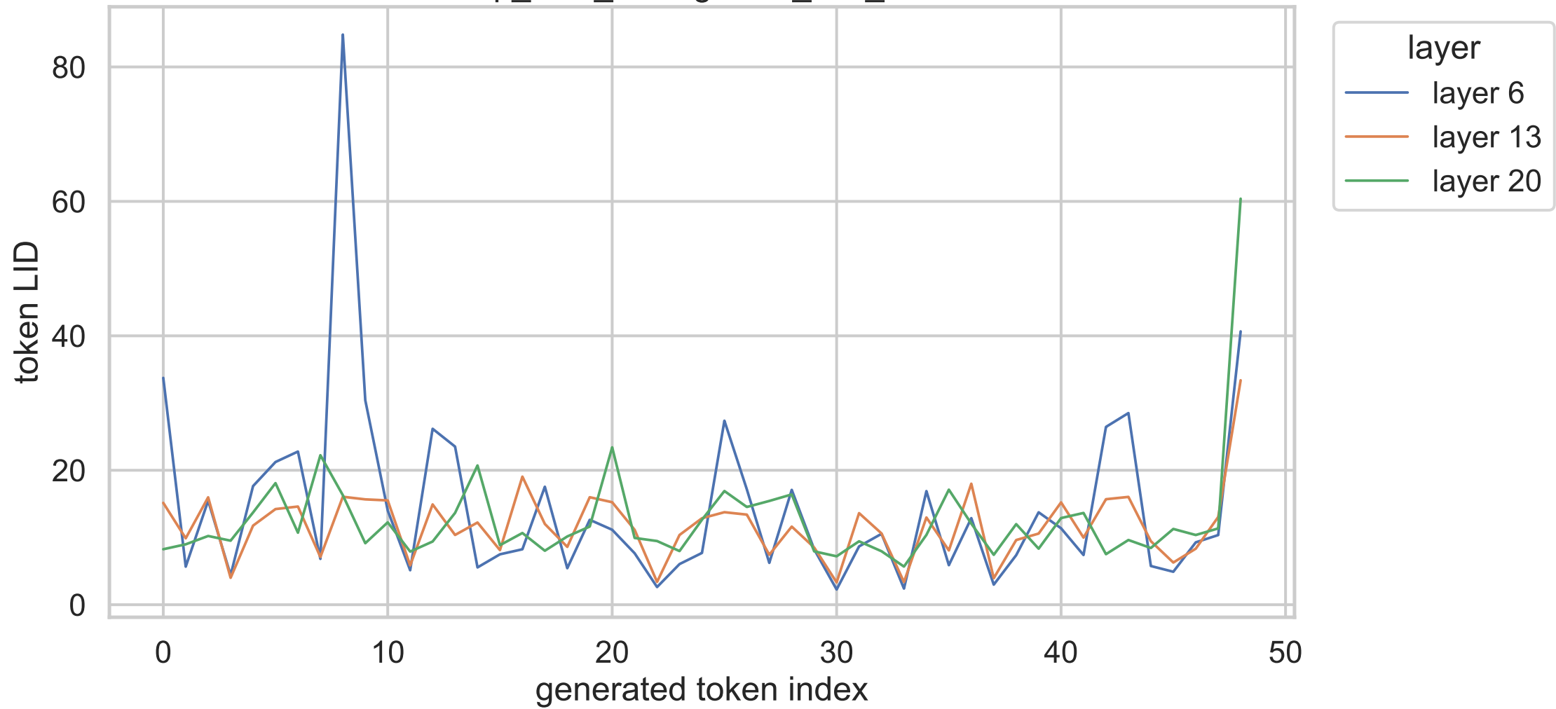
8B exp_c no_think gsm8k_test_001094
