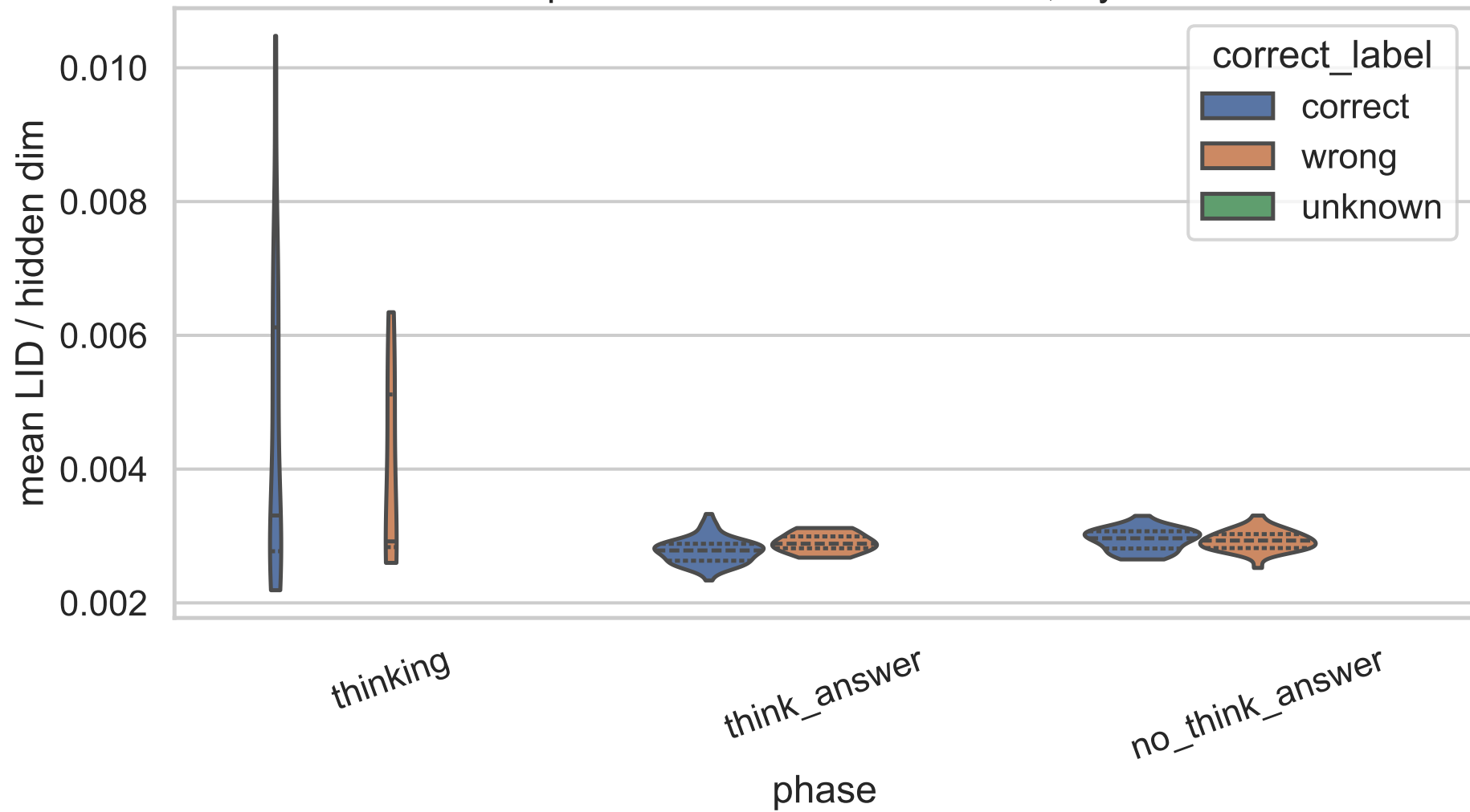
8B Exp C correctness-stratified LID, layer 20
