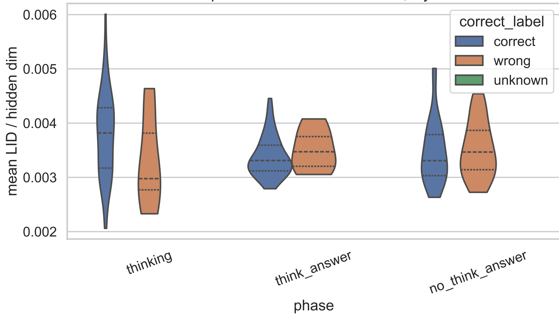
8B Exp C correctness-stratified LID, layer 6
