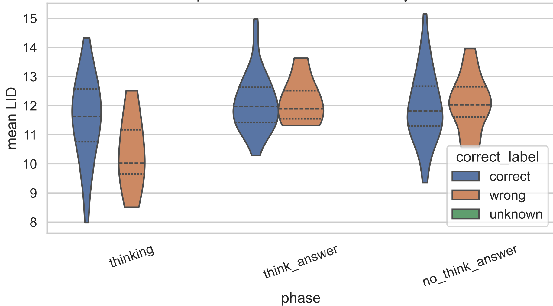
8B Exp C correctness-stratified LID, layer 13
