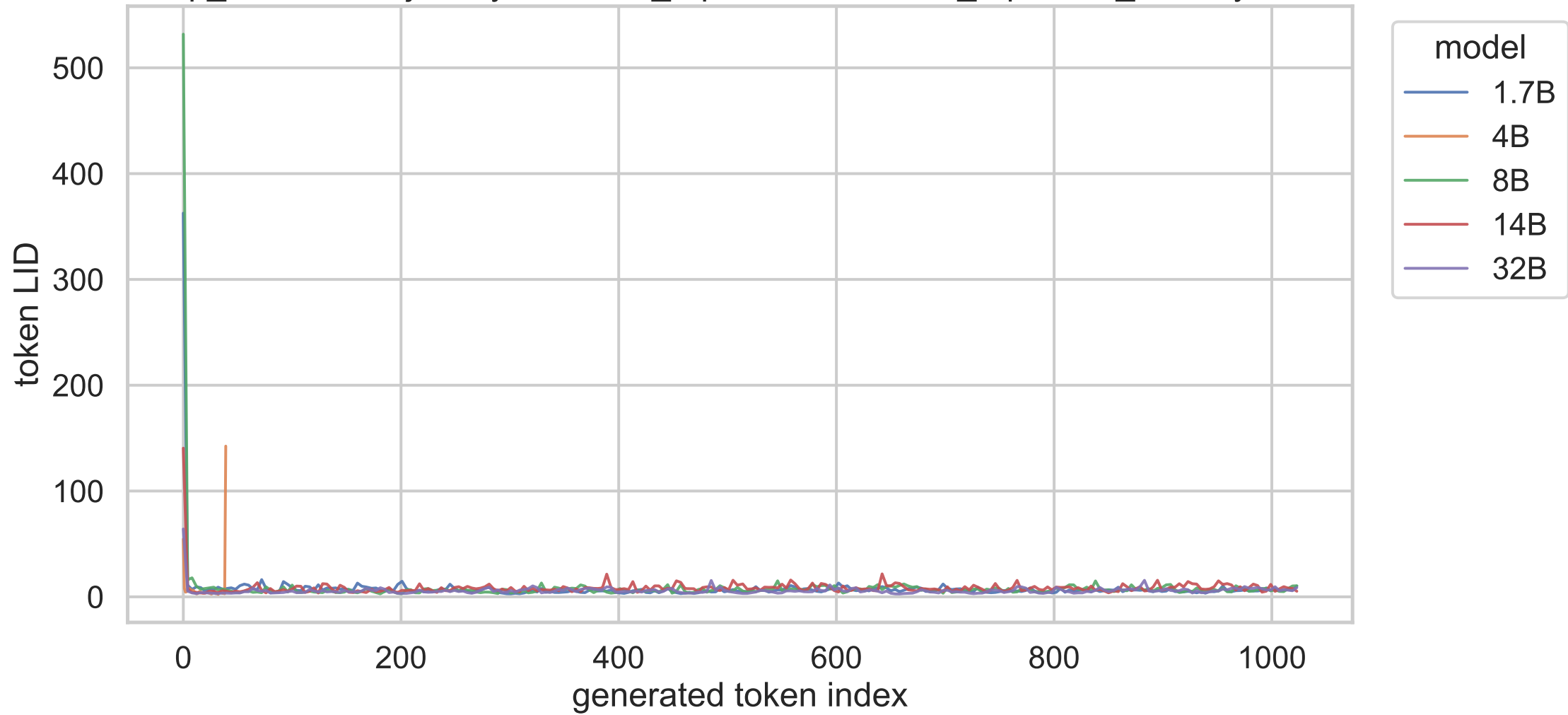
exp_a shared trajectory, constant_repetition, constant_repetition_null, layer 13
