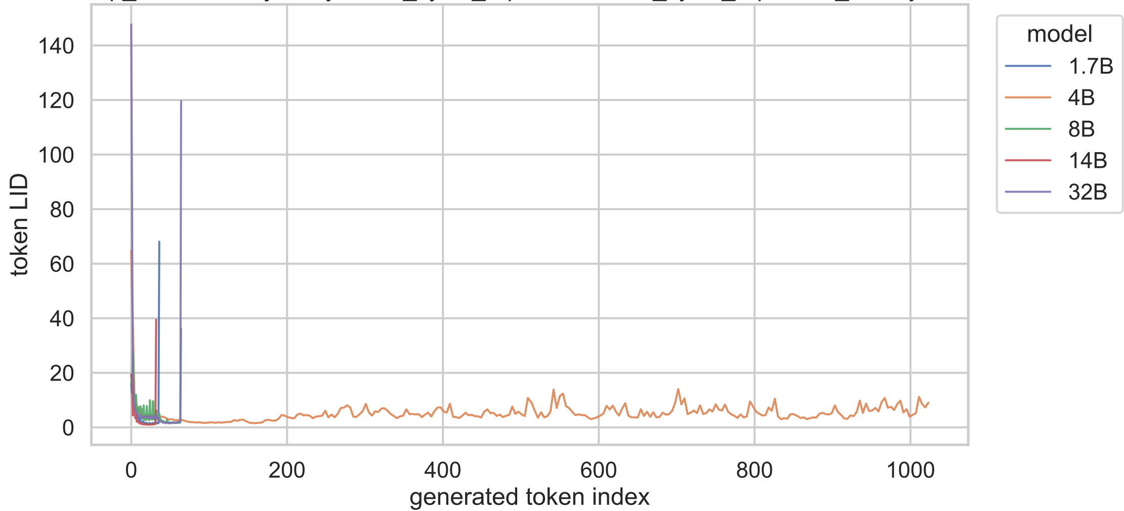
exp_a shared trajectory, short_cycle_repetition, short_cycle_repetition_02, layer 13
