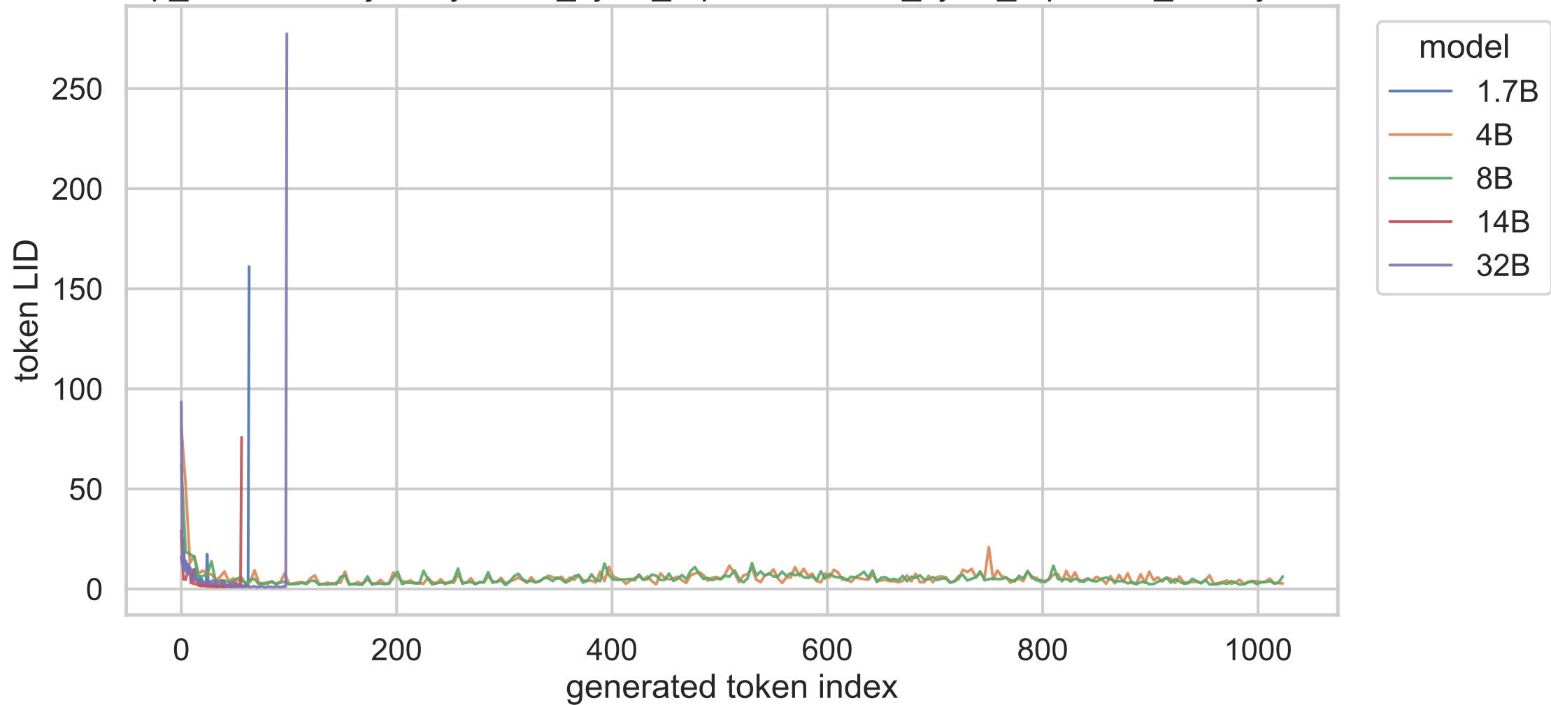
exp_a shared trajectory, short_cycle_repetition, short_cycle_repetition_03, layer 13
