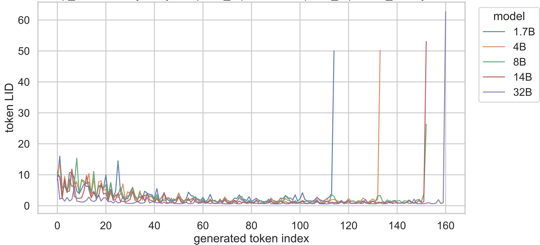
exp_a shared trajectory, templatic_repetition, templatic_repetition_03, layer 13
