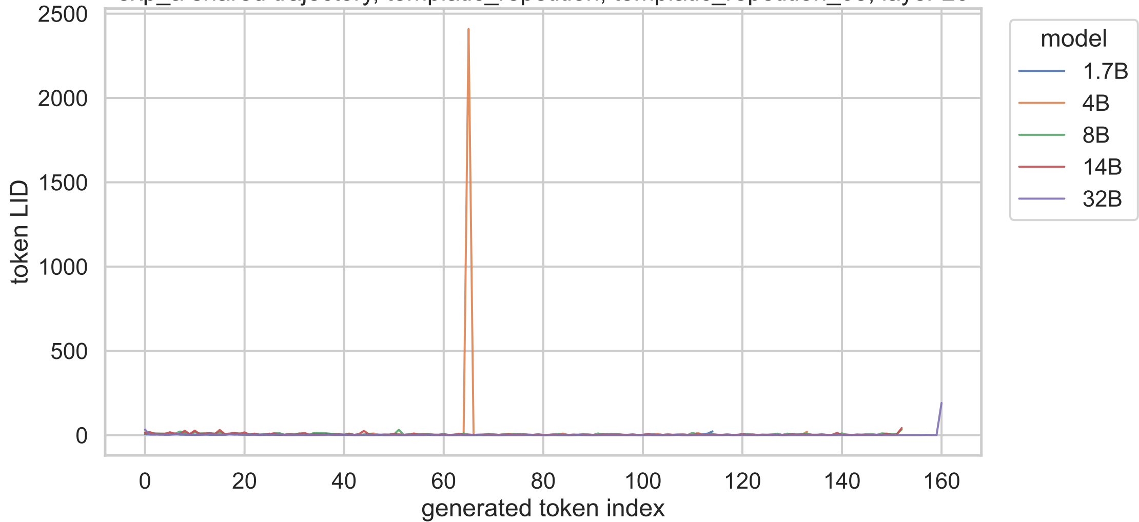
exp_a shared trajectory, templatic_repetition, templatic_repetition_03, layer 20
