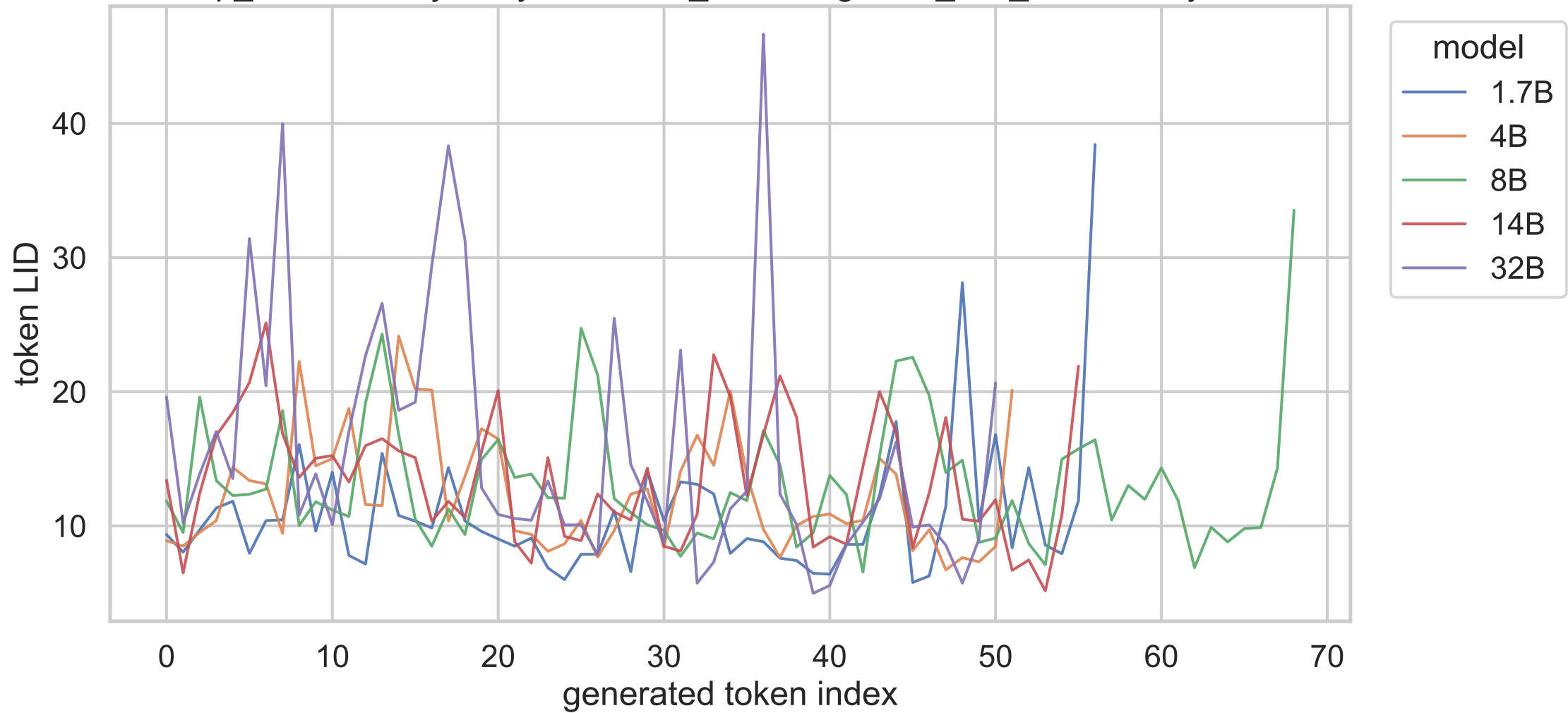
exp_b shared trajectory, irrelevant_context, gsm8k_test_000052, layer 20
