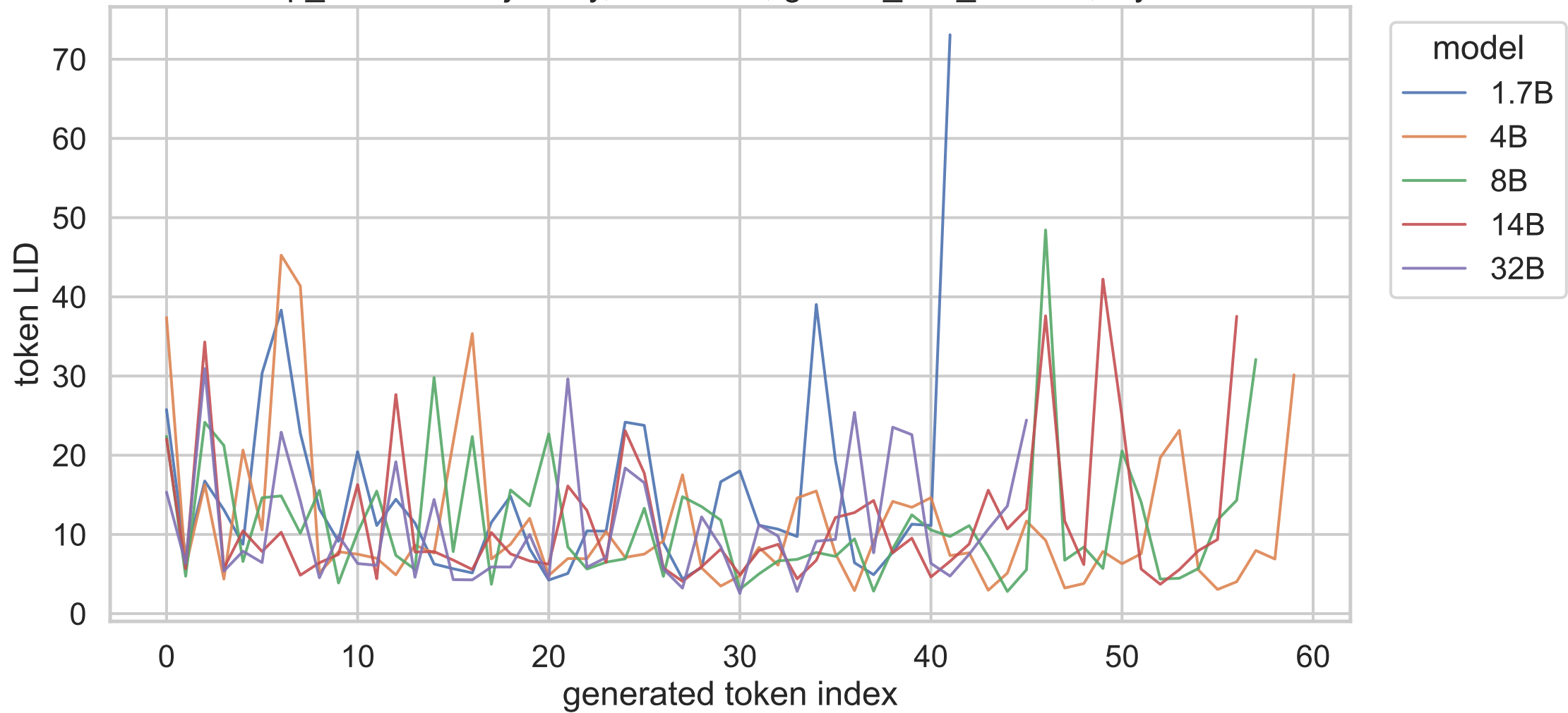
exp_b shared trajectory, canonical, gsm8k_test_000003, layer 6
