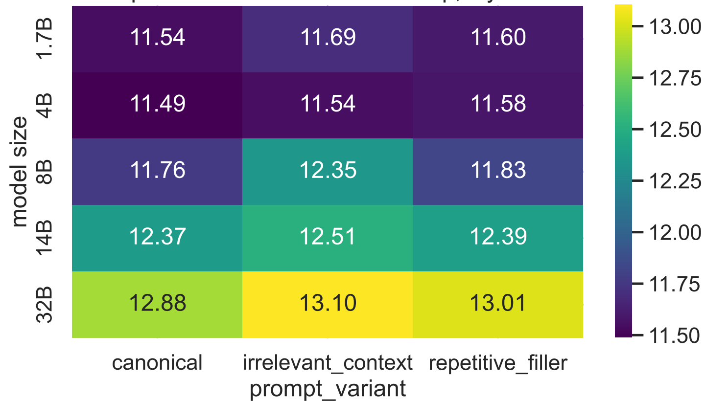
Exp B mean answer LID heatmap, layer 20
