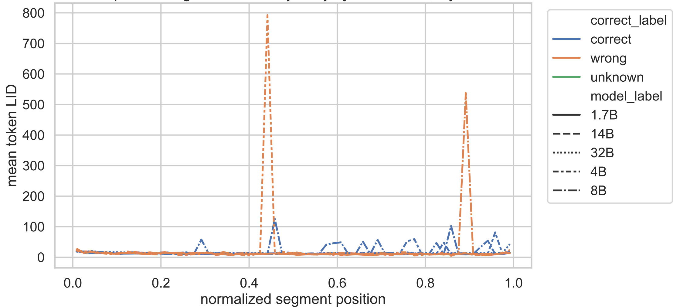
Exp C thinking normalized trajectory by correctness, layer 20
