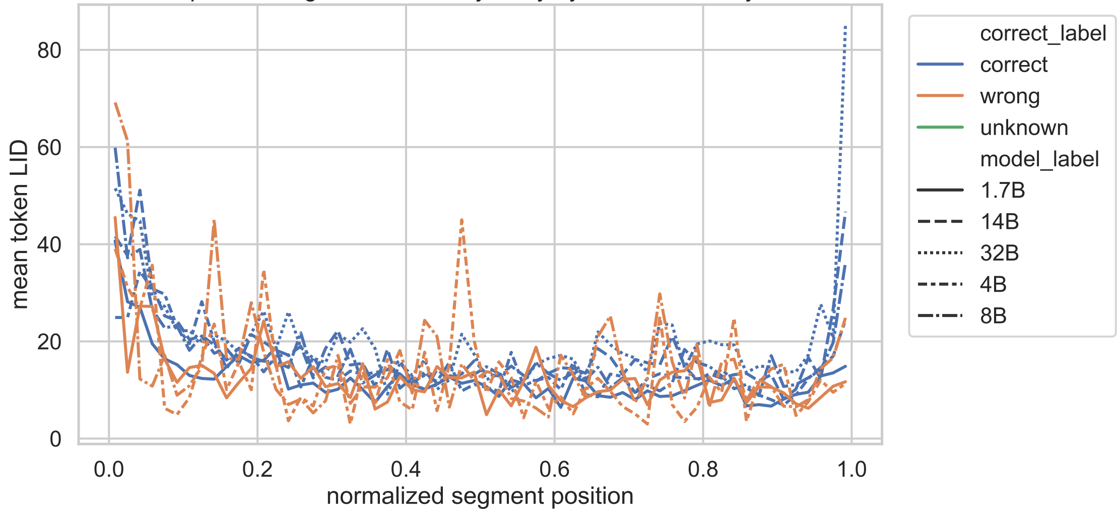
Exp C thinking normalized trajectory by correctness, layer 6
