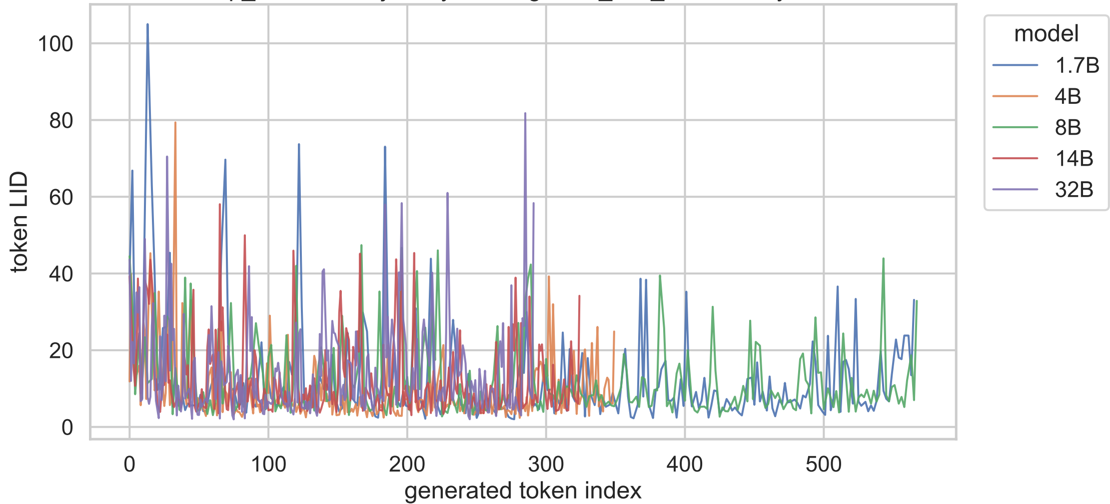
exp_c shared trajectory, think, gsm8k_test_000054, layer 13
