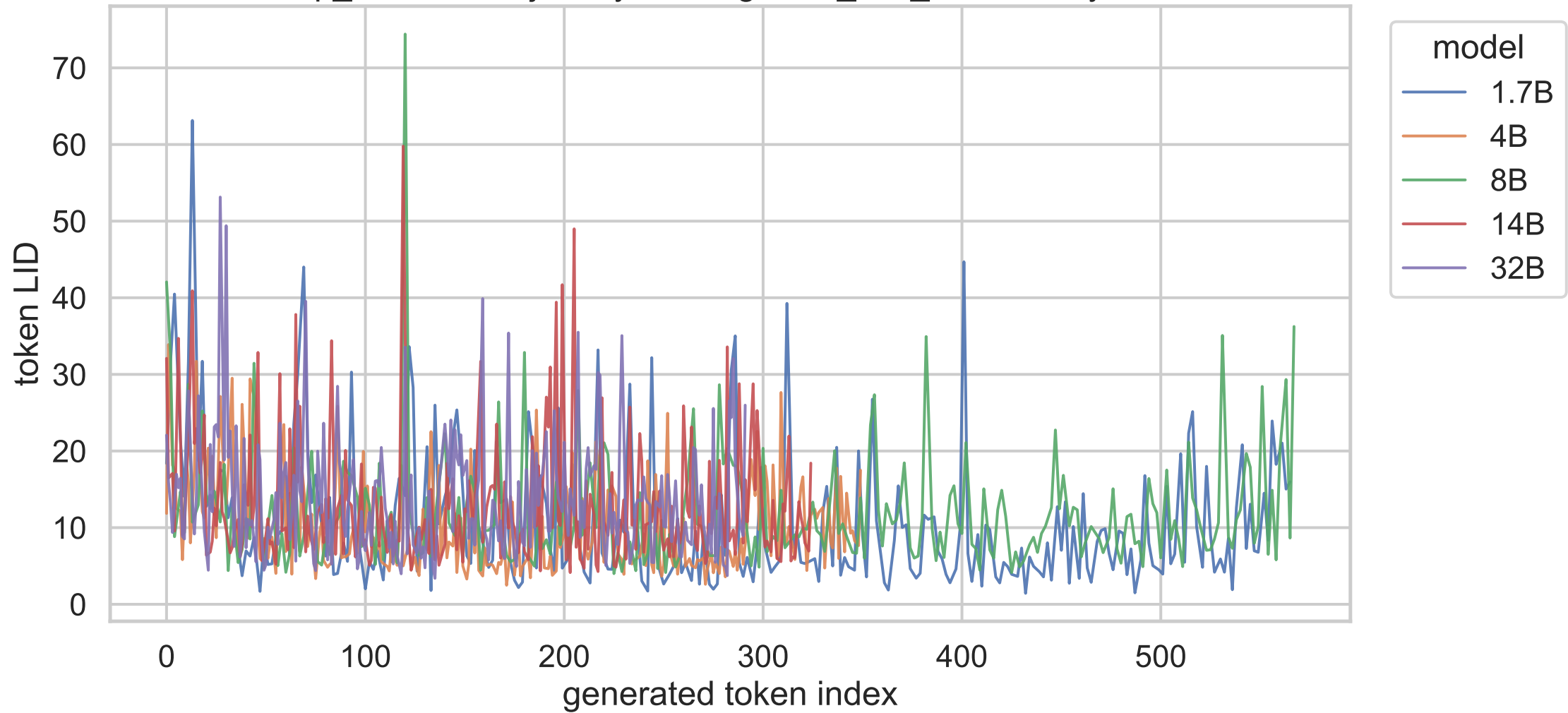
exp_c shared trajectory, think, gsm8k_test_000054, layer 20
