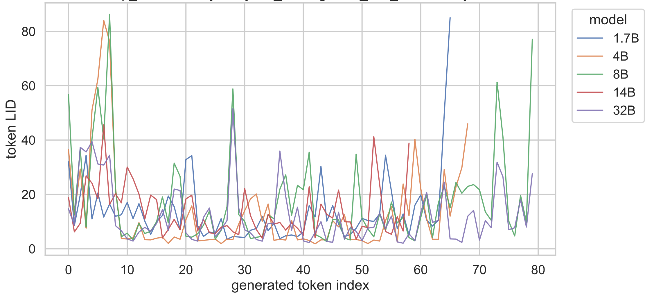
exp_c shared trajectory, no_think, gsm8k_test_000031, layer 6
