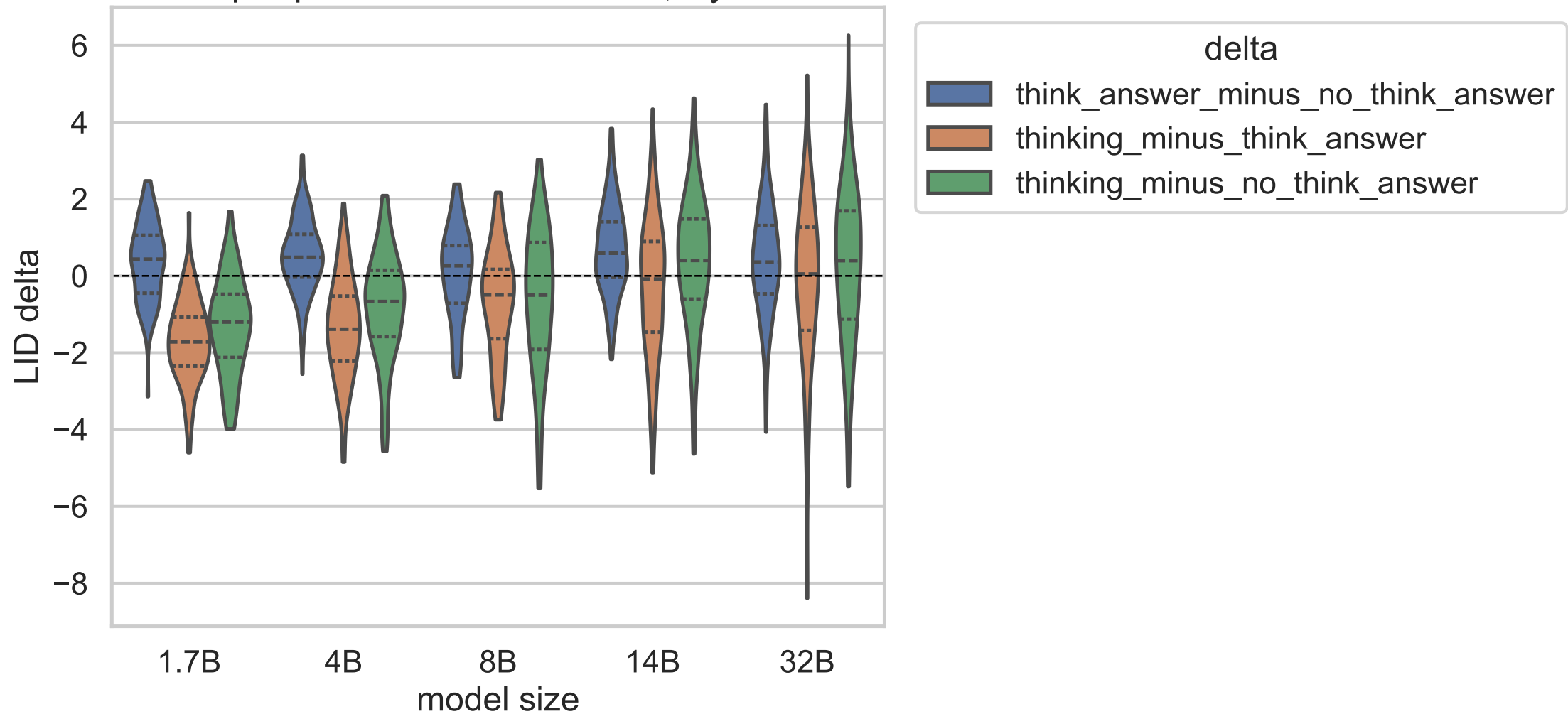
Exp C paired delta distributions, layer 13
