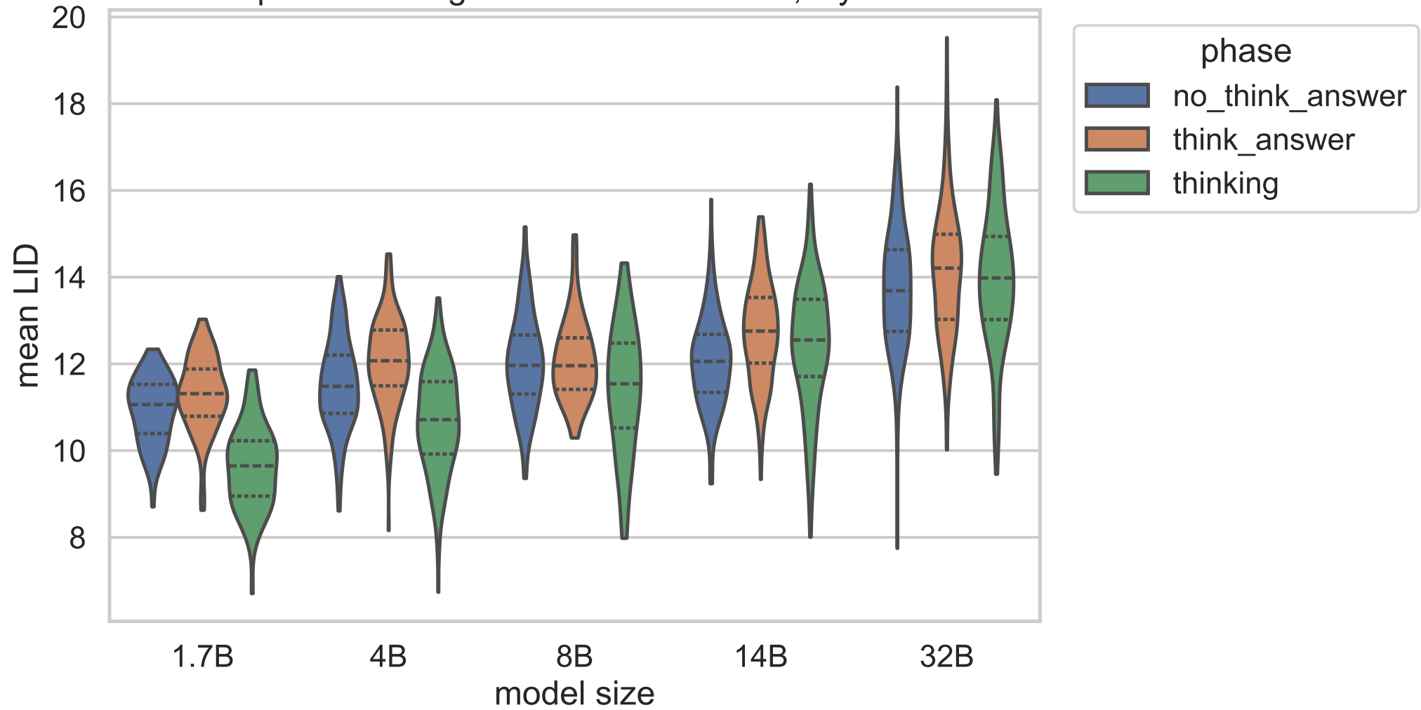
Exp C mean segment LID distributions, layer 13
