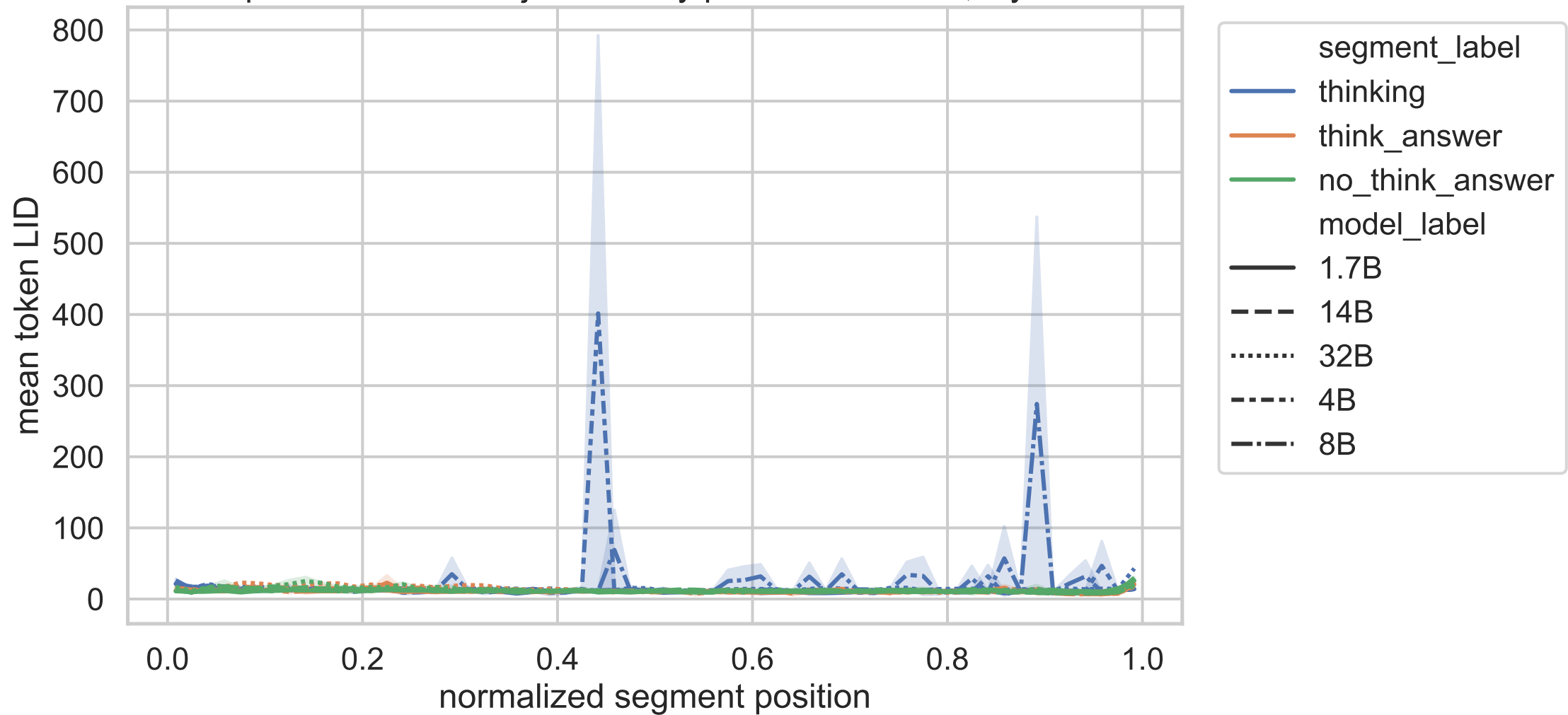
Exp C normalized trajectories by phase and model, layer 20
