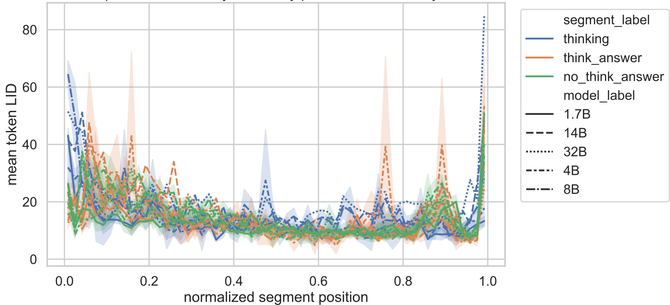
Exp C normalized trajectories by phase and model, layer 6
