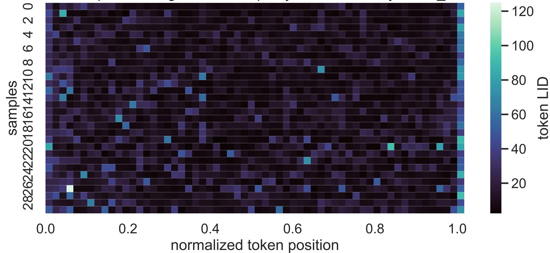
14B Exp C thinking LID heatmap, layer 13, sorted by mean_lid
