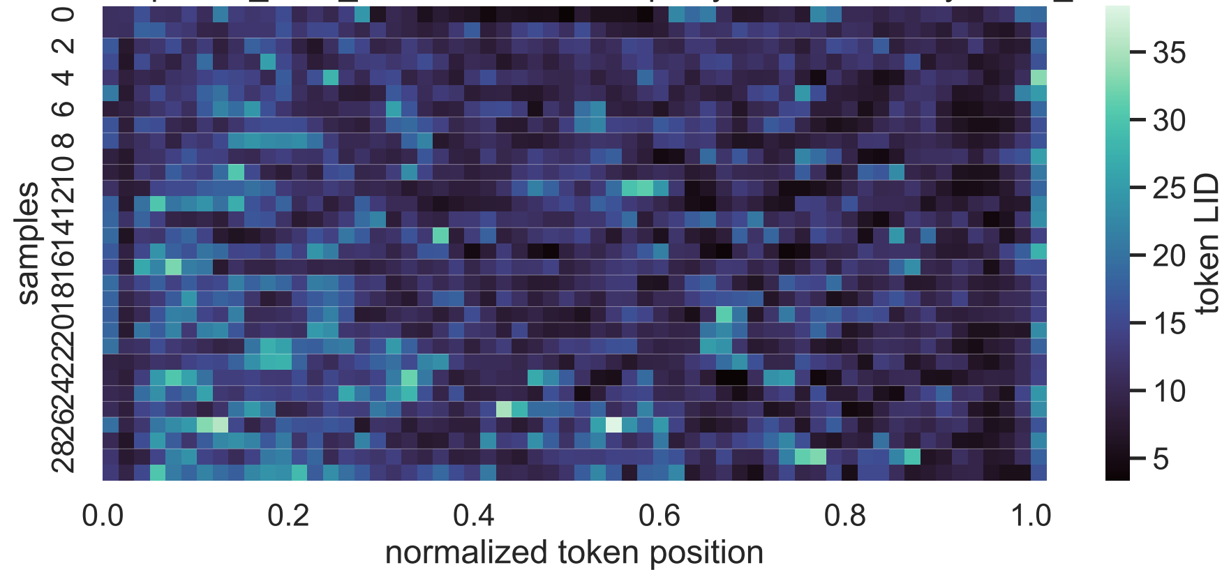
14B Exp C no_think_answer LID heatmap, layer 20, sorted by mean_lid
