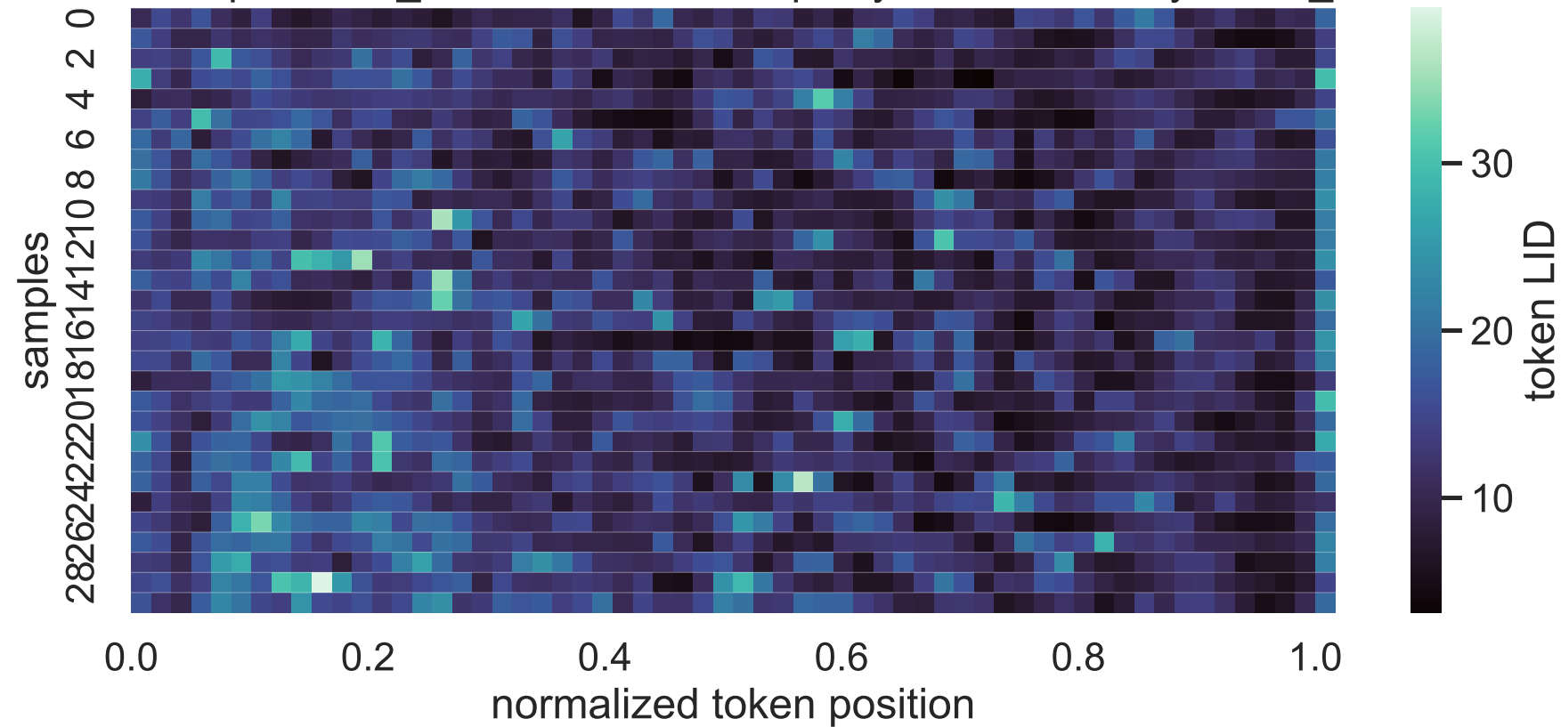
14B Exp C think_answer LID heatmap, layer 20, sorted by mean_lid
