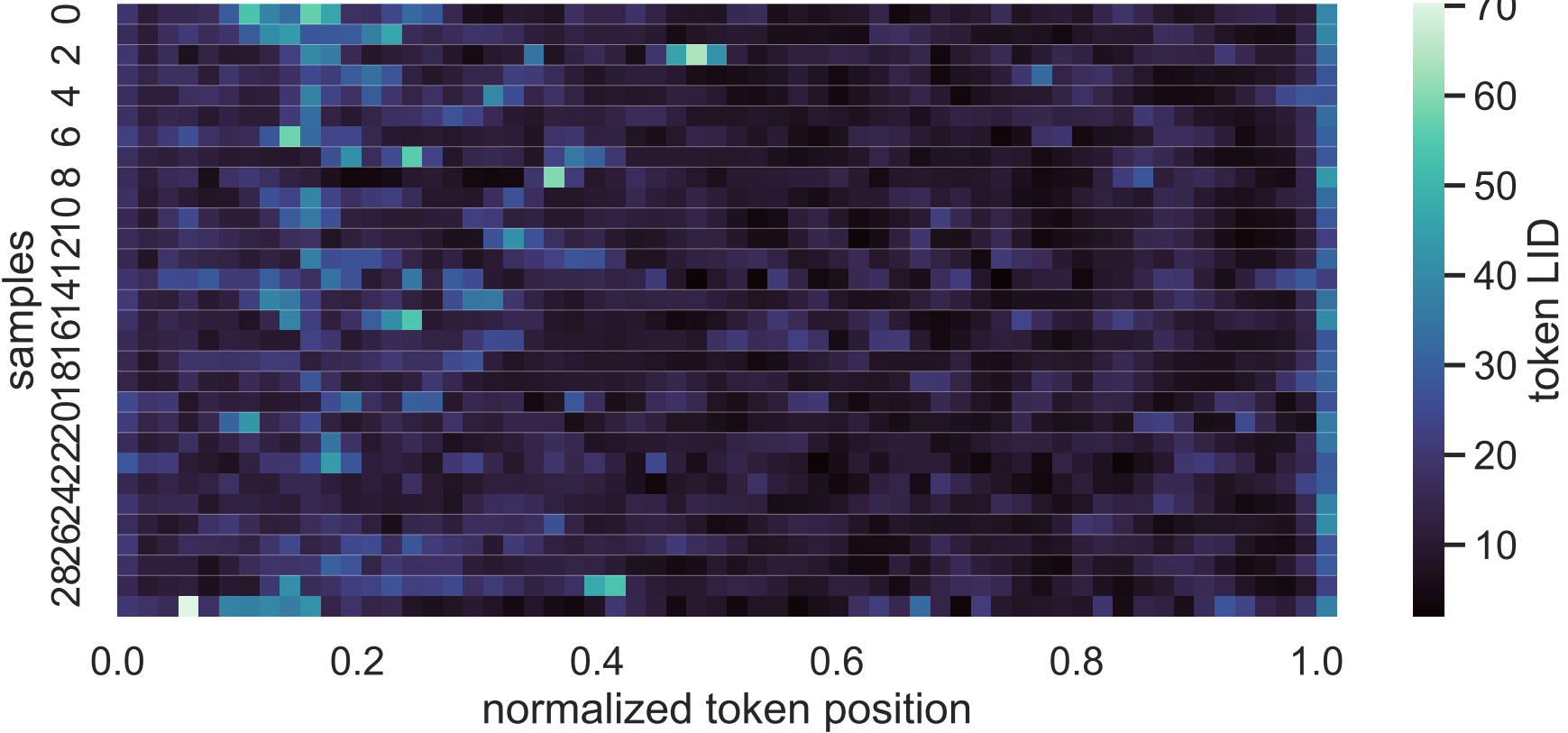
32B Exp C no_think_answer LID heatmap, layer 13, sorted by paired_delta
