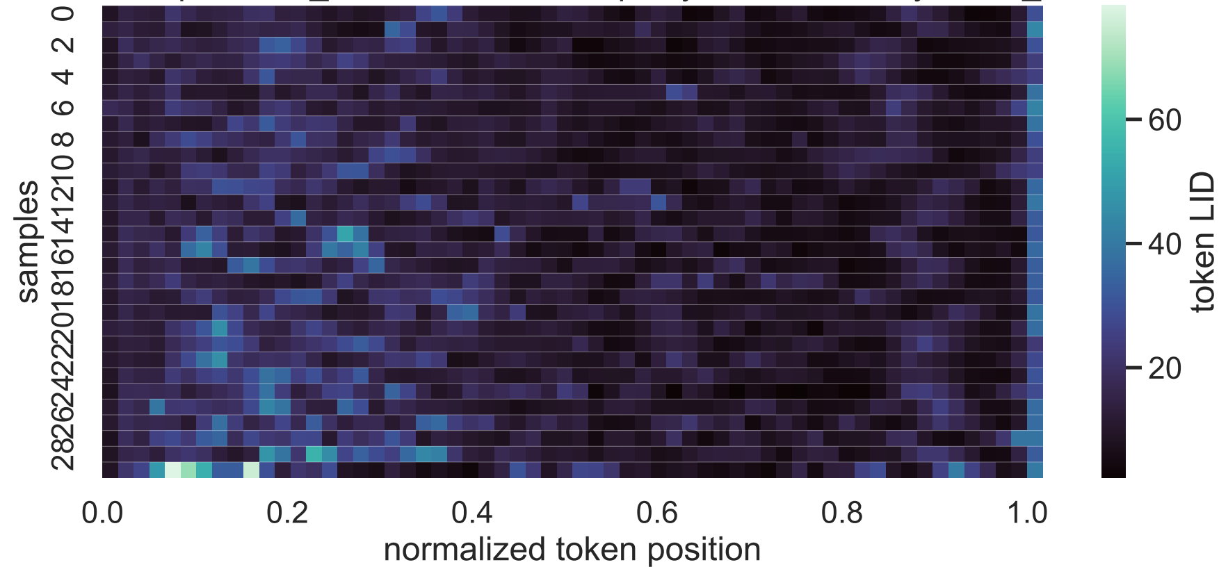
32B Exp C think_answer LID heatmap, layer 13, sorted by mean_lid
