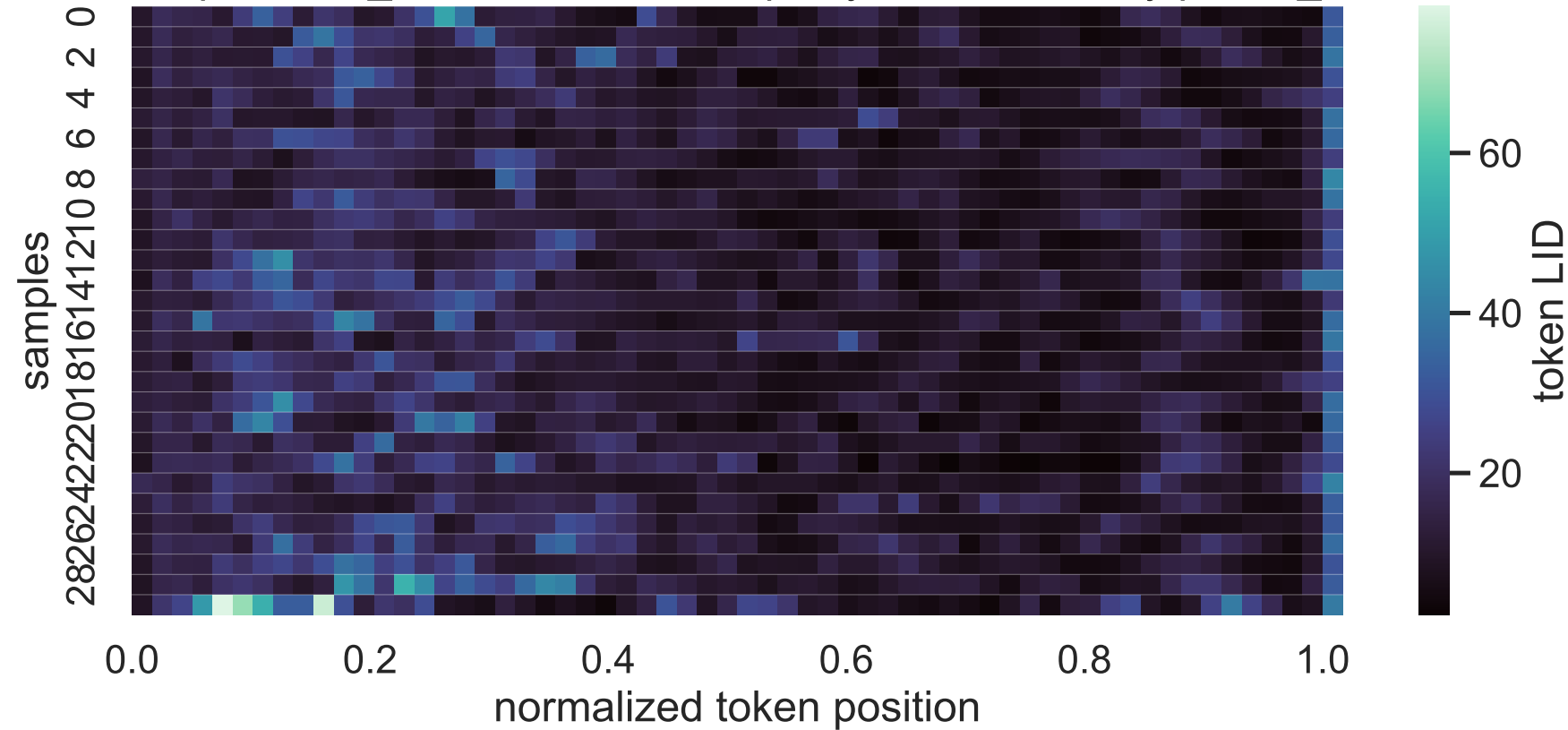
32B Exp C think_answer LID heatmap, layer 13, sorted by paired_delta
