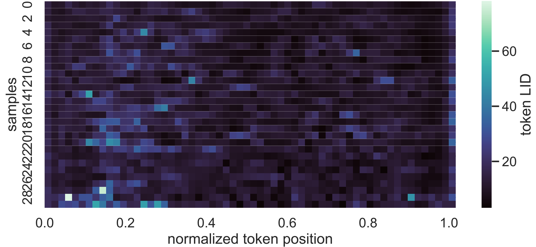
32B Exp C no_think_answer LID heatmap, layer 20, sorted by correctness_then_mean_lid
