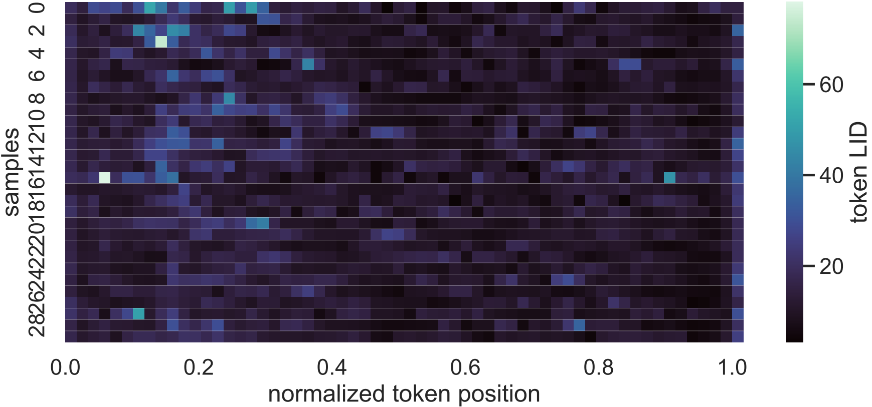
32B Exp C no_think_answer LID heatmap, layer 20, sorted by paired_delta
