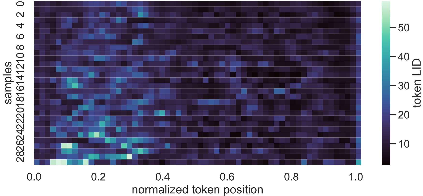
32B Exp C think_answer LID heatmap, layer 20, sorted by correctness_then_mean_lid
