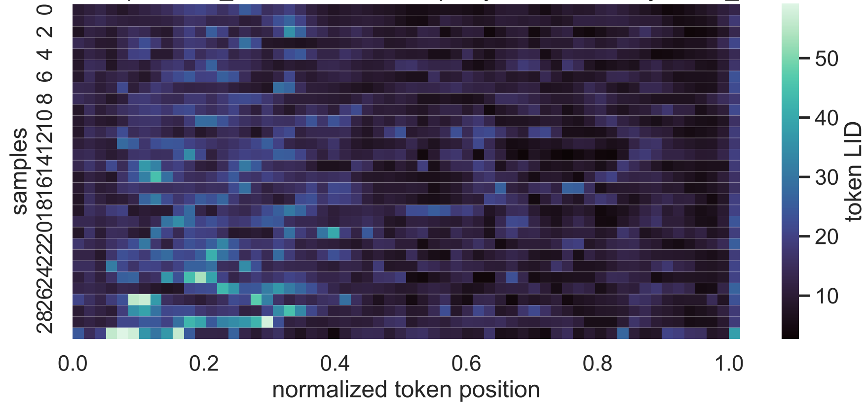
32B Exp C think_answer LID heatmap, layer 20, sorted by mean_lid
