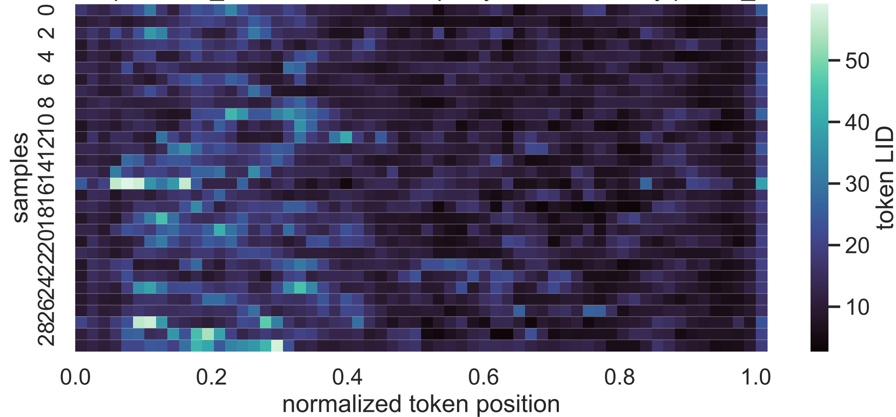
32B Exp C think_answer LID heatmap, layer 20, sorted by paired_delta
