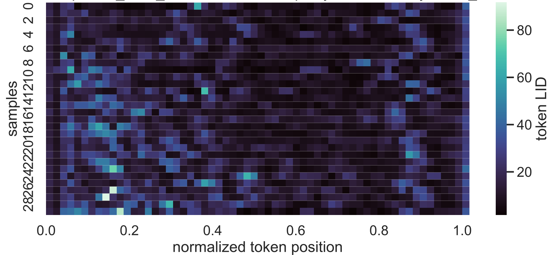
32B Exp C no_think_answer LID heatmap, layer 6, sorted by mean_lid
