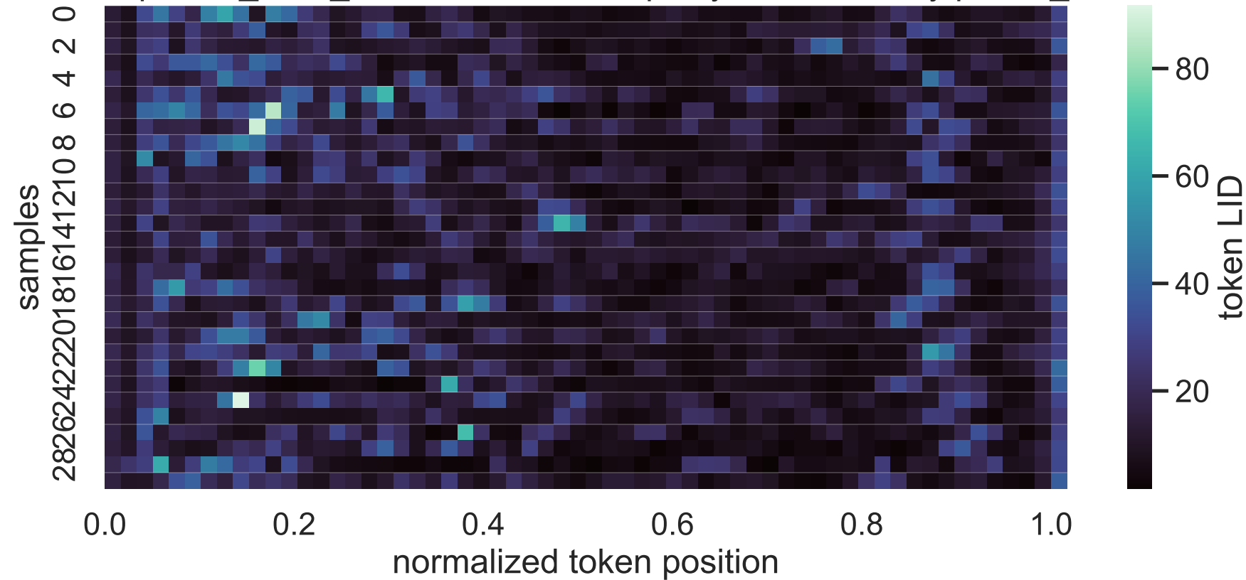
32B Exp C no_think_answer LID heatmap, layer 6, sorted by paired_delta
