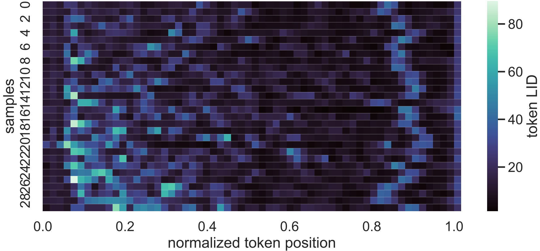
32B Exp C think_answer LID heatmap, layer 6, sorted by correctness_then_mean_lid
