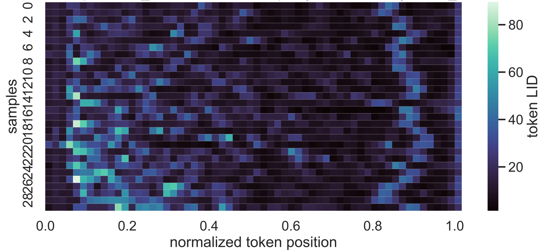
32B Exp C think_answer LID heatmap, layer 6, sorted by mean_lid
