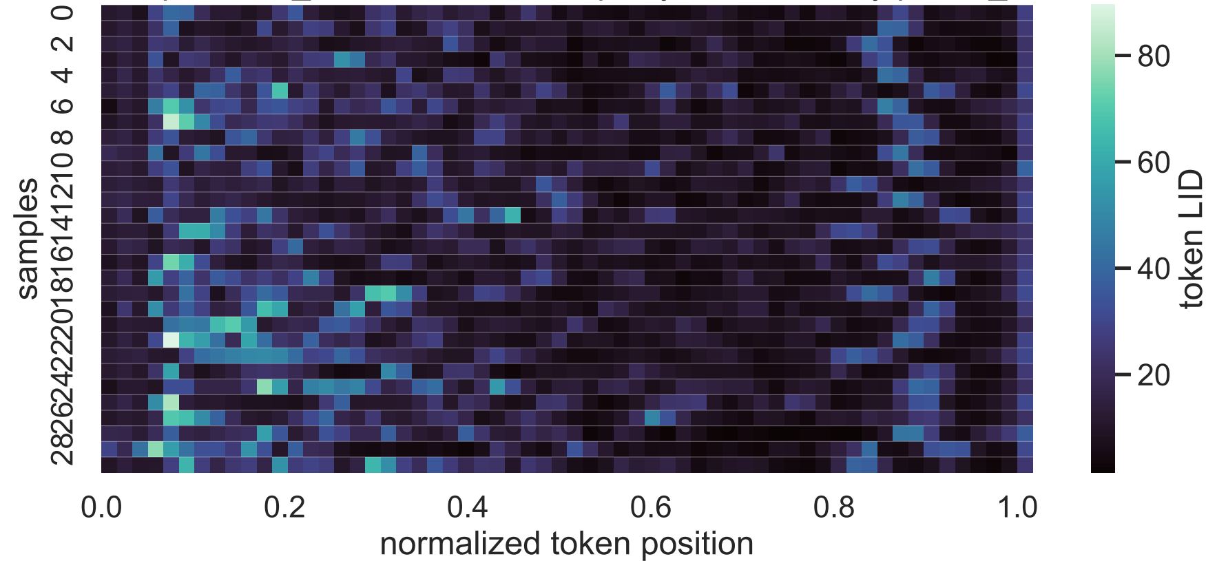
32B Exp C think_answer LID heatmap, layer 6, sorted by paired_delta
