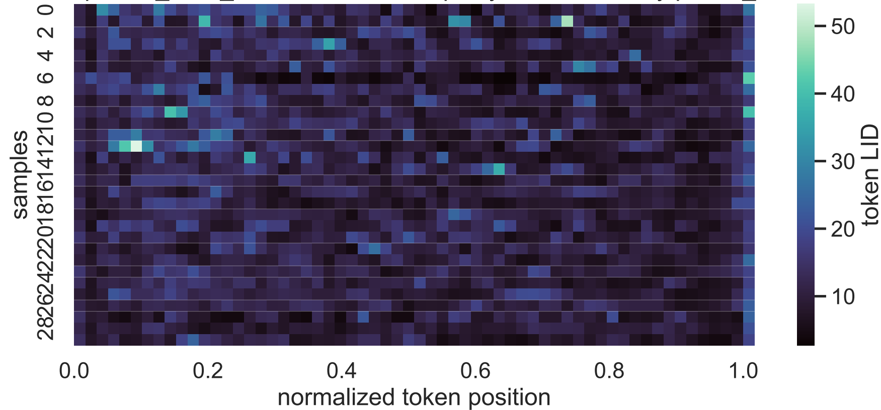
4B Exp C no_think_answer LID heatmap, layer 13, sorted by paired_delta
