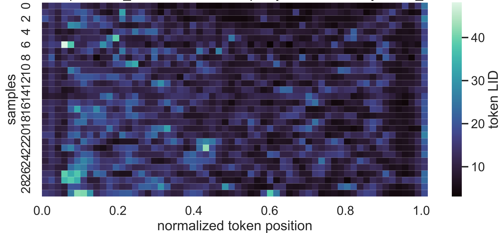
4B Exp C think_answer LID heatmap, layer 13, sorted by mean_lid
