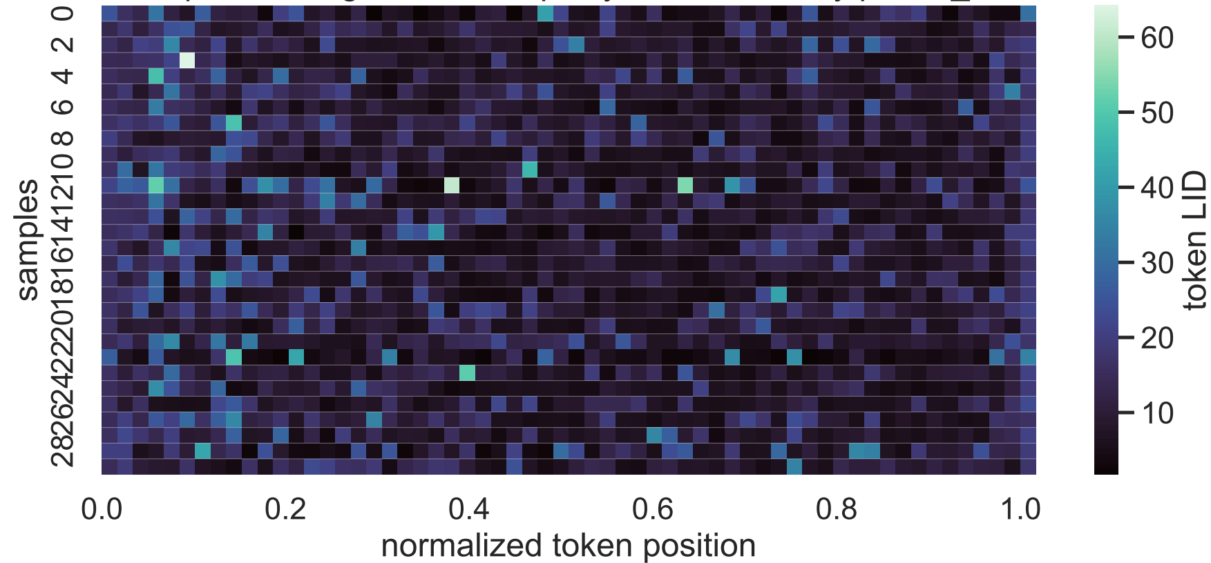
4B Exp C thinking LID heatmap, layer 13, sorted by paired_delta
