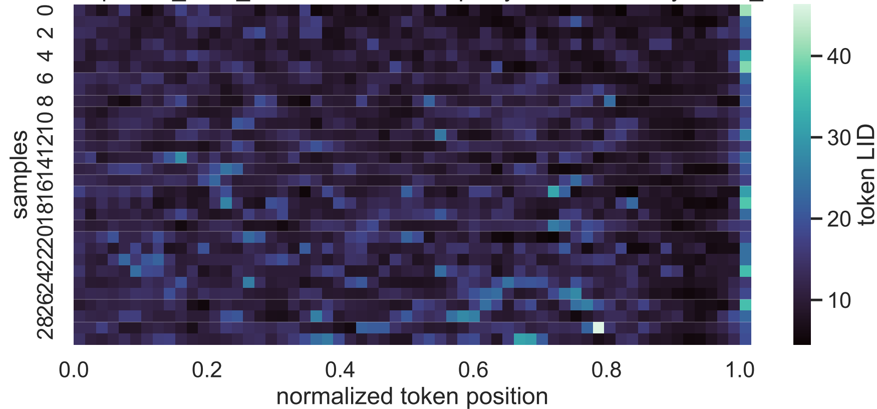
4B Exp C no_think_answer LID heatmap, layer 20, sorted by mean_lid
