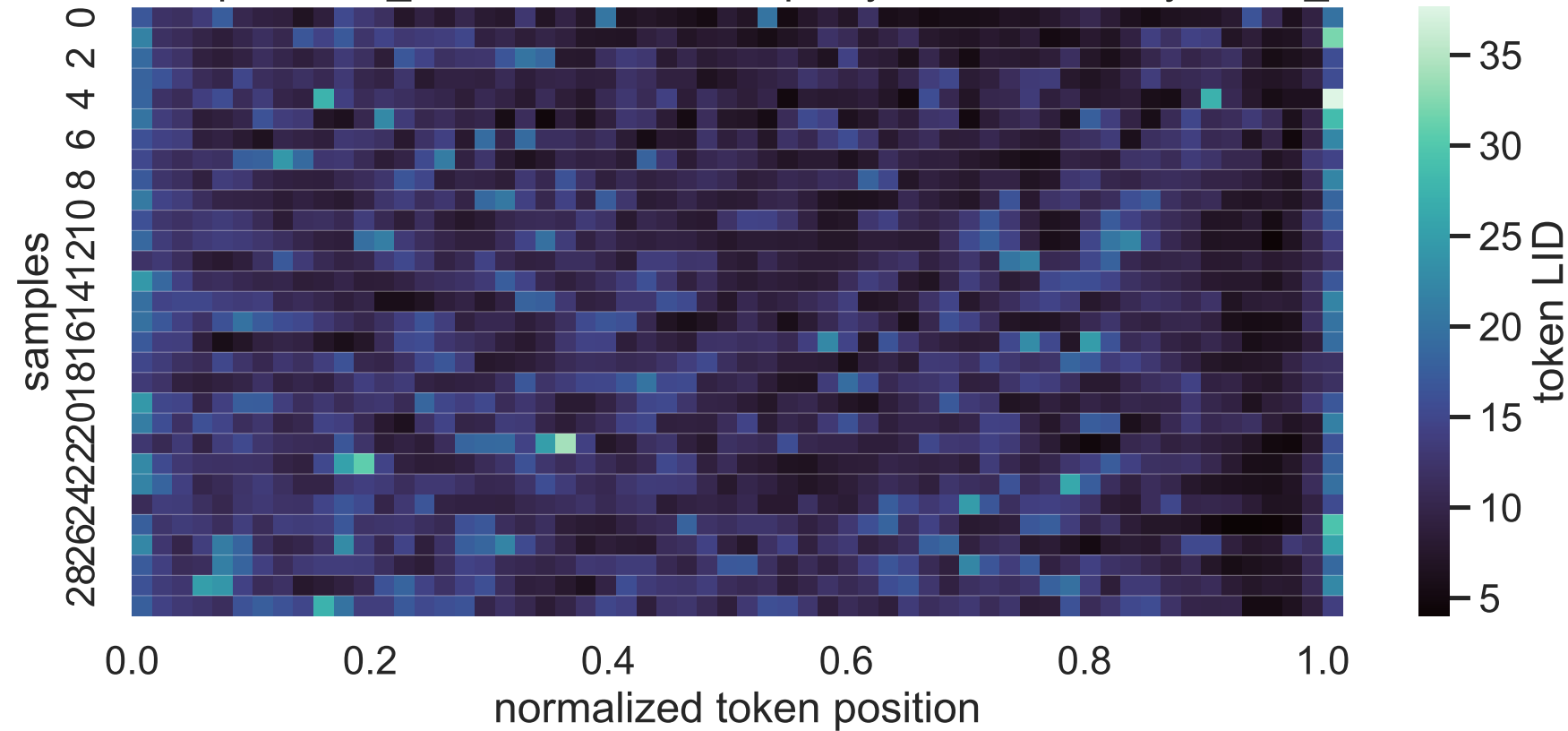
4B Exp C think_answer LID heatmap, layer 20, sorted by mean_lid
